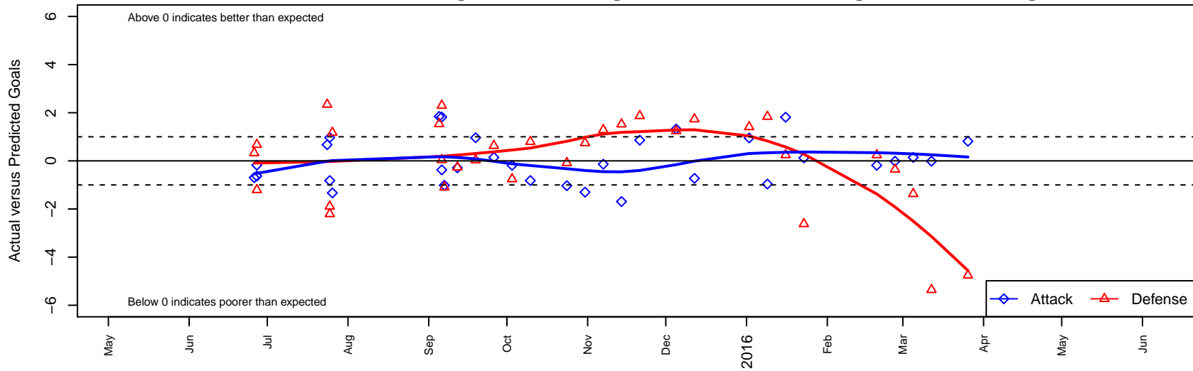
Crossfire Select Taylor B01 Dots are actual minus expected GF (blue circles) and GA (red triangles). Blue line is smoothed change in attack strength. Red is smoothed change in defense strength.
